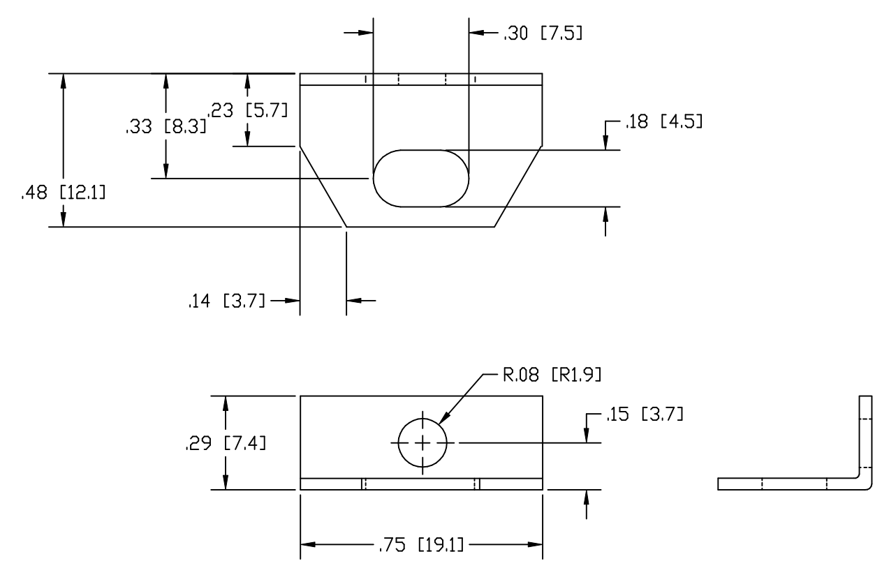
MINI MOUNTING CLIP DIMENSIONS (NOT TO SCALE)
